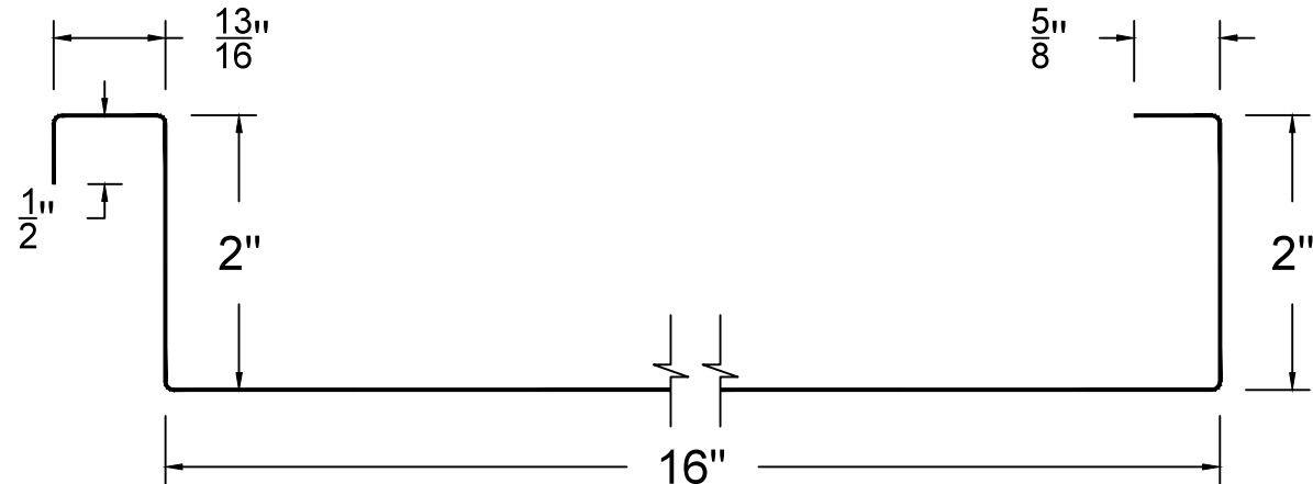
PANEL PROFILE
