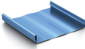
Striations
